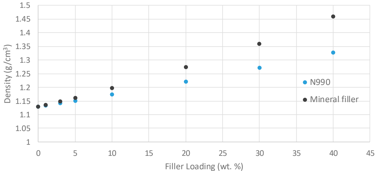
Figure 7. Density of polyamide composites as a function of filler loading. At high loadings, weight savings of greater than 10% can be realized by using N990 over mineral fillers.
