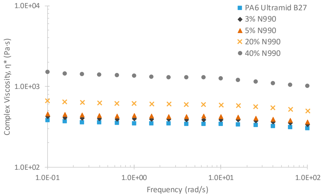
Figure 1. Complex viscosity curves at varying frequency and 240°C. As N990 loading increased, viscosity also increased. There was no significant viscosity change up to 5 wt.% N990 loading.
